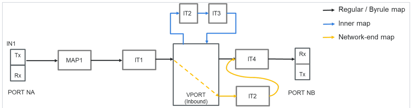
Figure 15 Flexible Inline Decryption Maps
